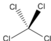
Carbon Tetrachloride
