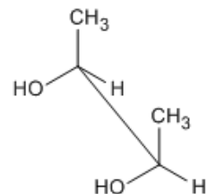
Sawhorse Projection (Stereochemistry)
