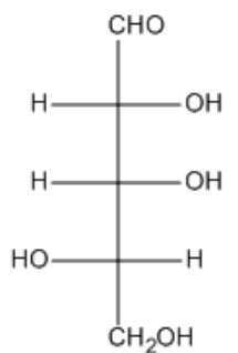
Fischer Projection (Sugars)
