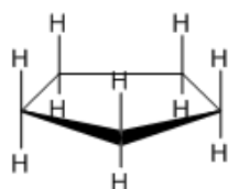
Haworth Projection (Cycloalkanes)
